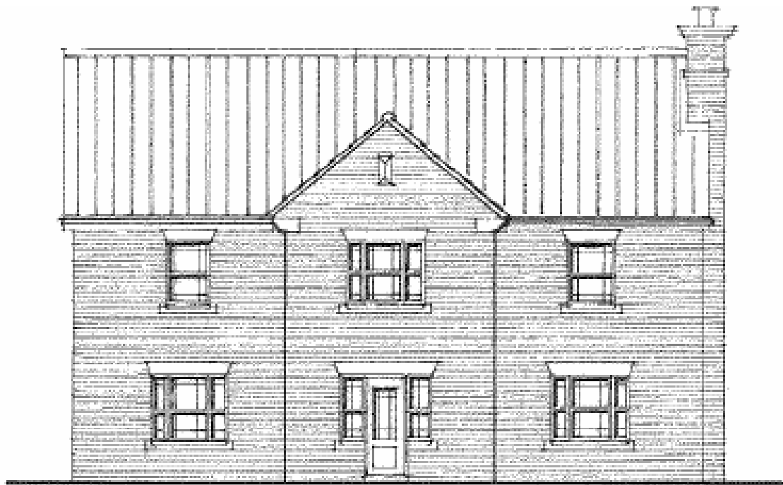
east elevation
