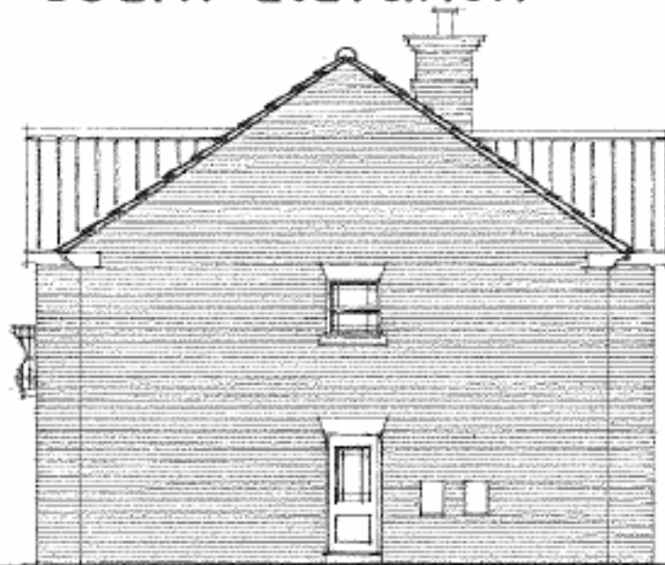
north elevation
